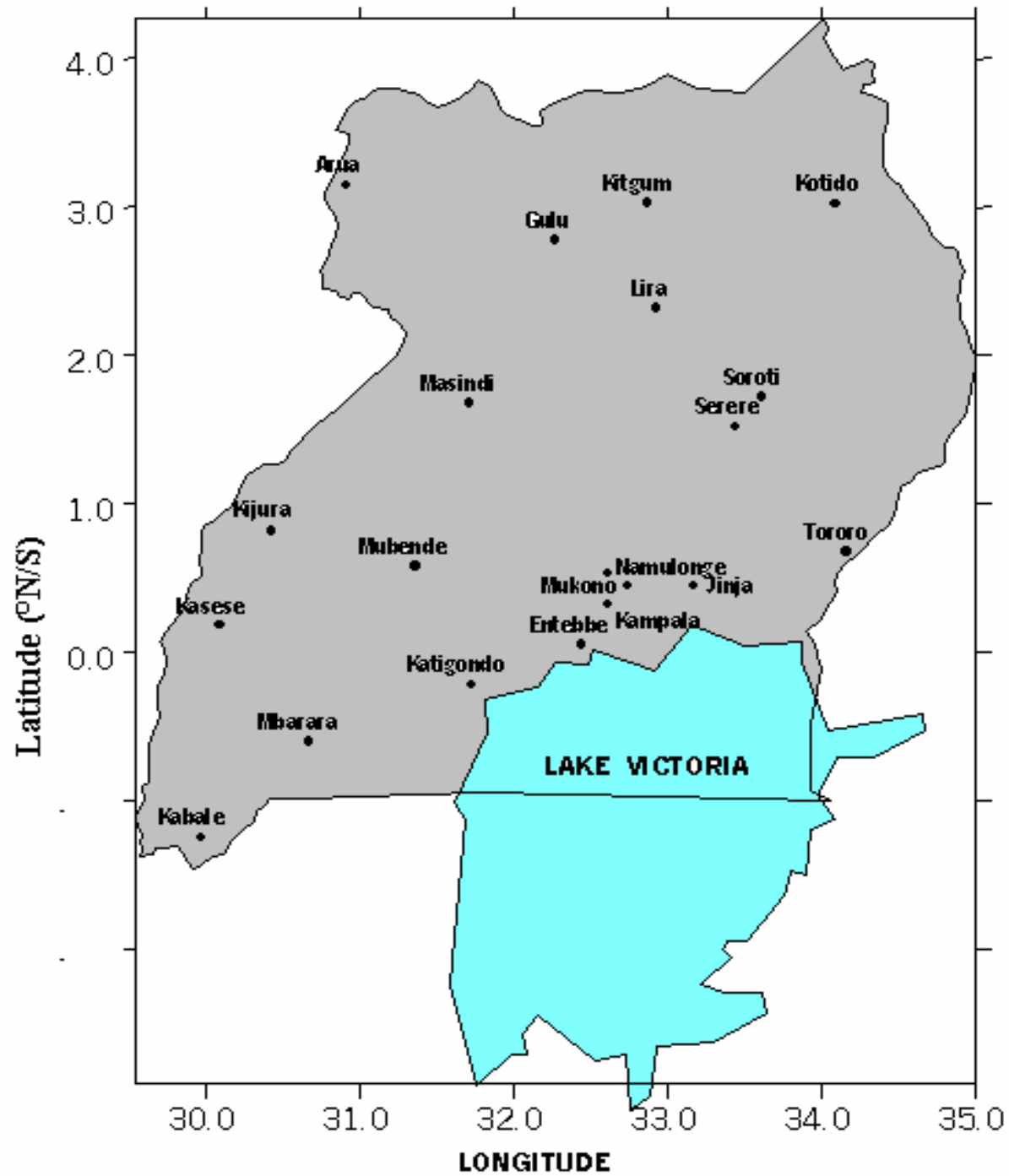
Rainfall Stations in Uganda
