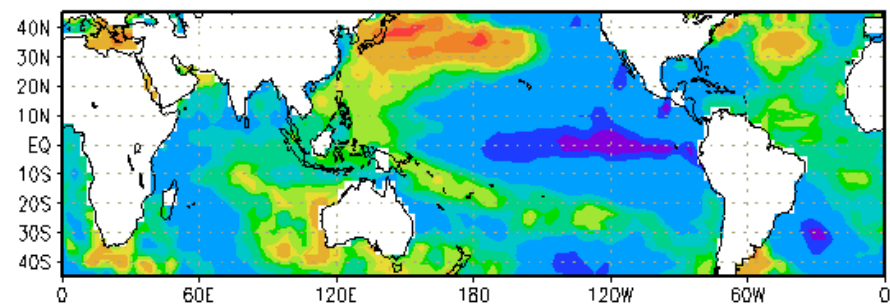
GLOBAL SST INDEX PATTERNS FOR A MATURE PHASE OF LA-NINA
