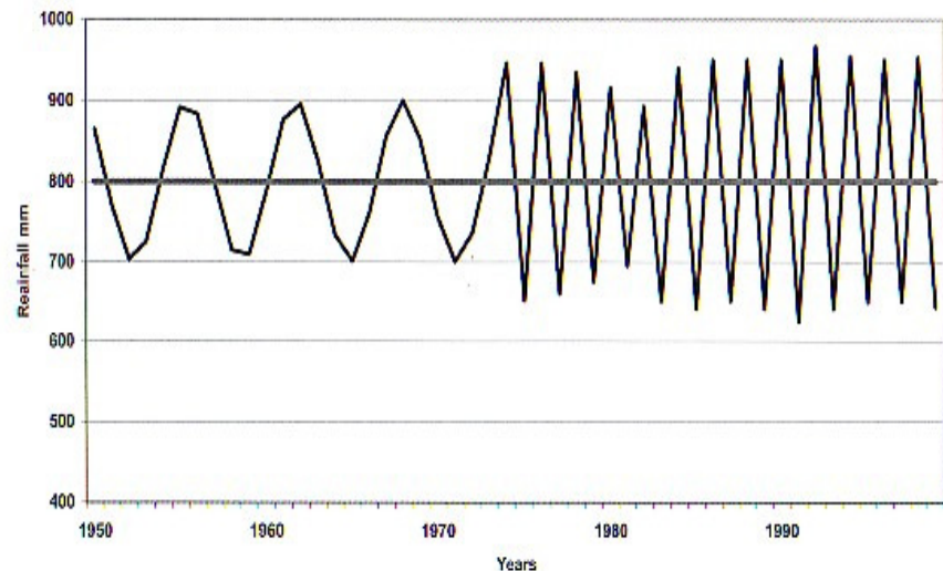
Change in frequency of Extremes and magnitude of extremes
