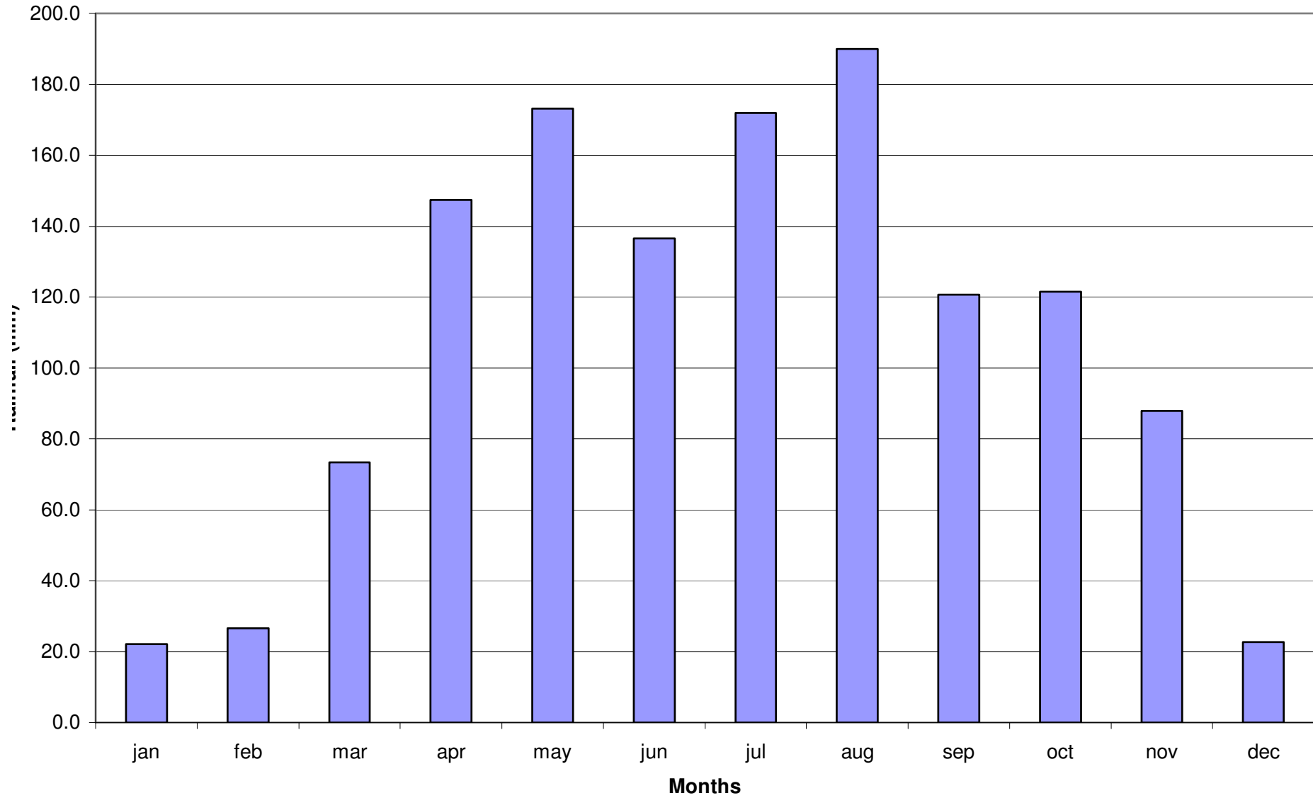
Mean Monthly rainfall over Kitgum
