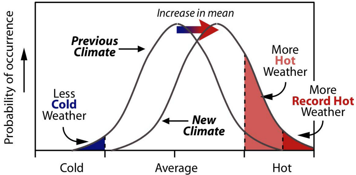
Change in Mean and Frequency
