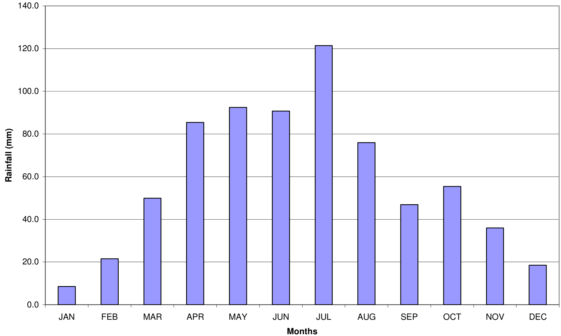
Monthly variation of Rainfall over Kotido
