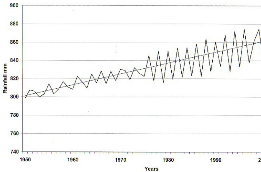
Change in Mean and Frequency
