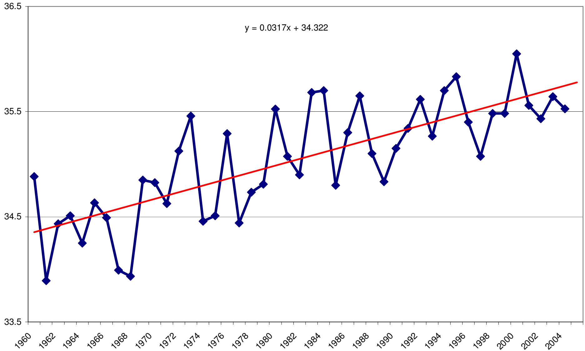
Mean Annual Maximum Temperature over Lodwar
