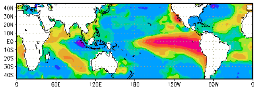
GLOBAL OCEAN SST INDEX PATTERNS FOR A MATURE PHASE OF EL-NINO
