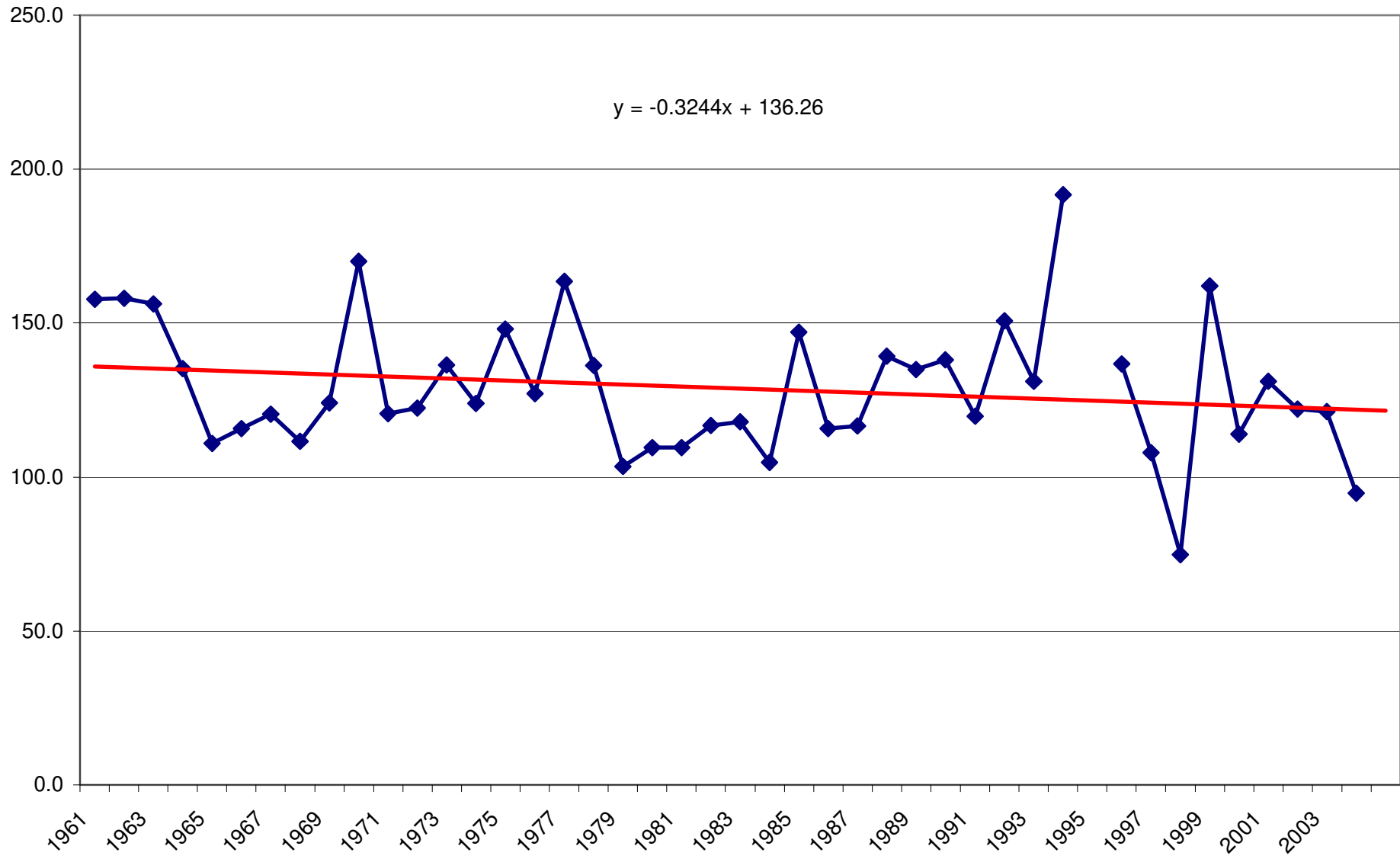
Mean Annual Rainfall over Gulu
