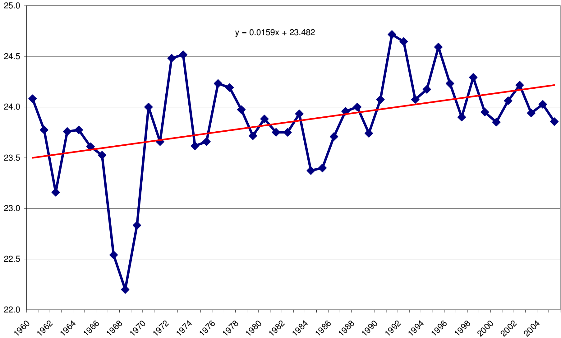
Mean Annual Minimum Temperature over Lodwar
