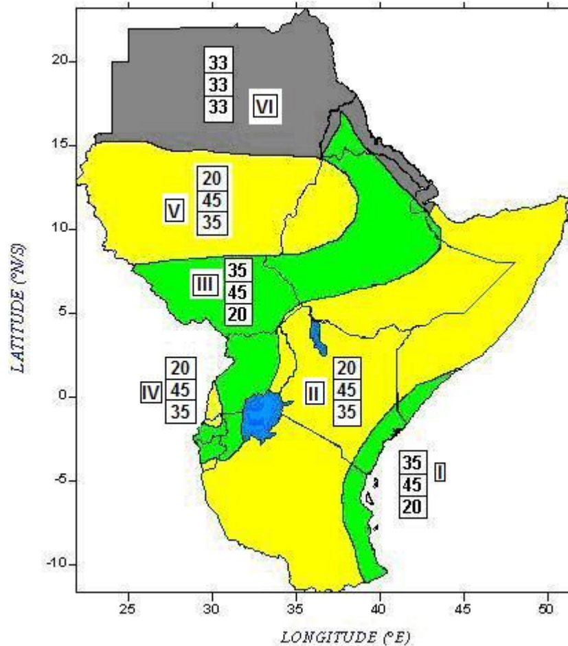
Consensus Climate Outlook for March –May 2007
