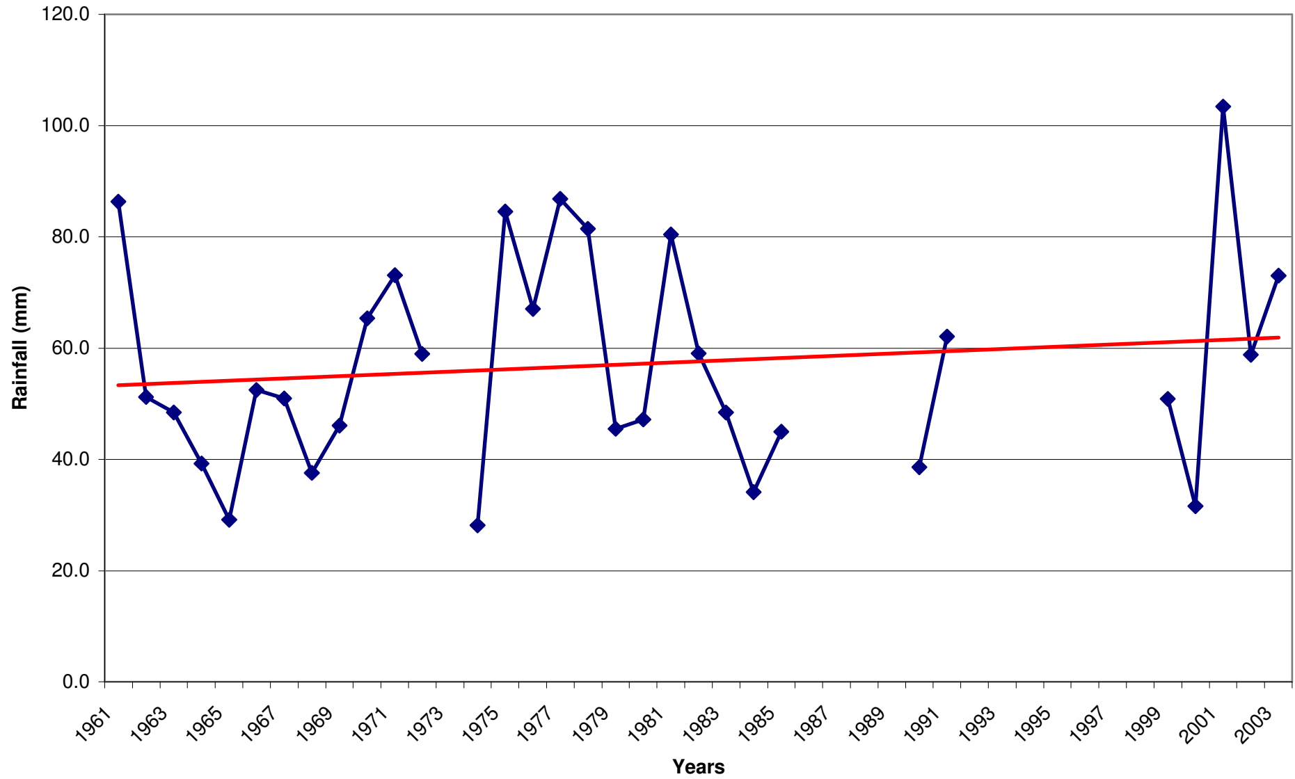
Variation of the Mean Annual rainfall over Kotido
